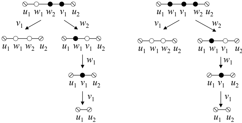
Figure 3. In the indicated two configurations, the neighbors of the \{w_1, w_2, v_1\} triplet, u_1 and u_2 , change color in the same way by pressing only v_1 and pressing w_2w_1v_1 . The color change on u_1 and u_2 is indicated with the flipping of their crossing line.
