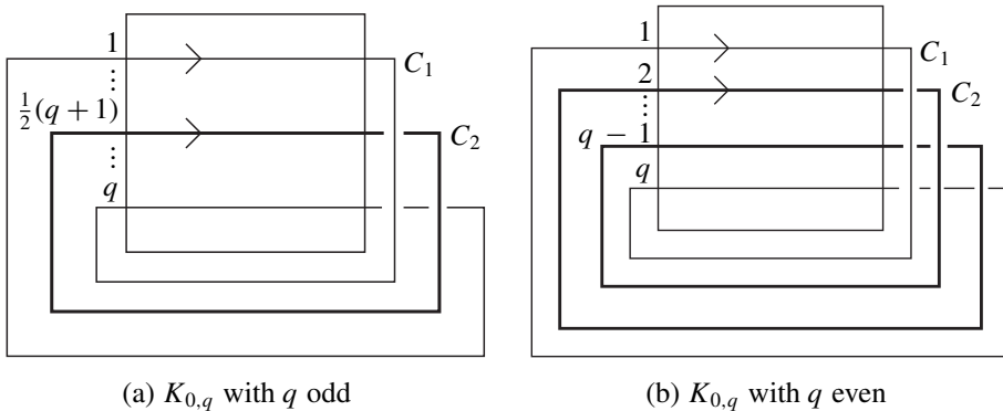
Figure 7. K_{0,q} .
