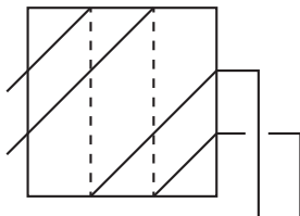
Figure 8. Two components of K_{n,n} on a single wrap.
