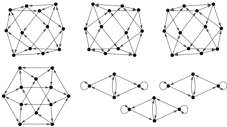
Figure 8. 2S(A_5; \{(235)\}, \{(243), (254)\}) .
