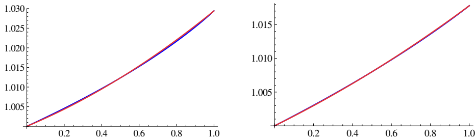
Figure 5. The error estimate E_{q_1}(f, x) when a = 0.9 and c increases from 4.1 to 6.1.
