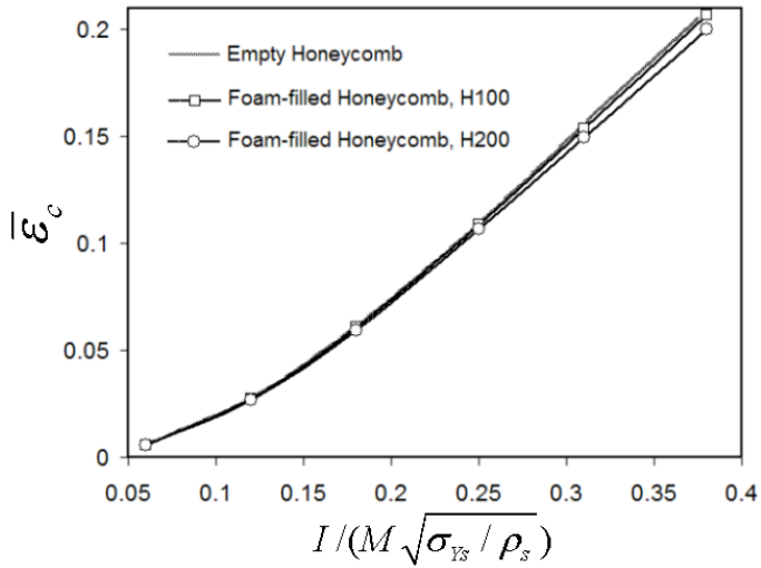
(b) The maximum nominal compressive strain in the core, \bar{\epsilon}_c , of empty and foam-filled square honeycomb sandwich plates versus normalized momentum impulse, I/(M\sqrt{\sigma_{Ys}/\rho_s}) .
