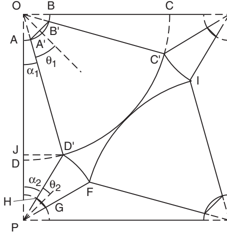
Figure 10. Geometry of variable angle wedge field.
