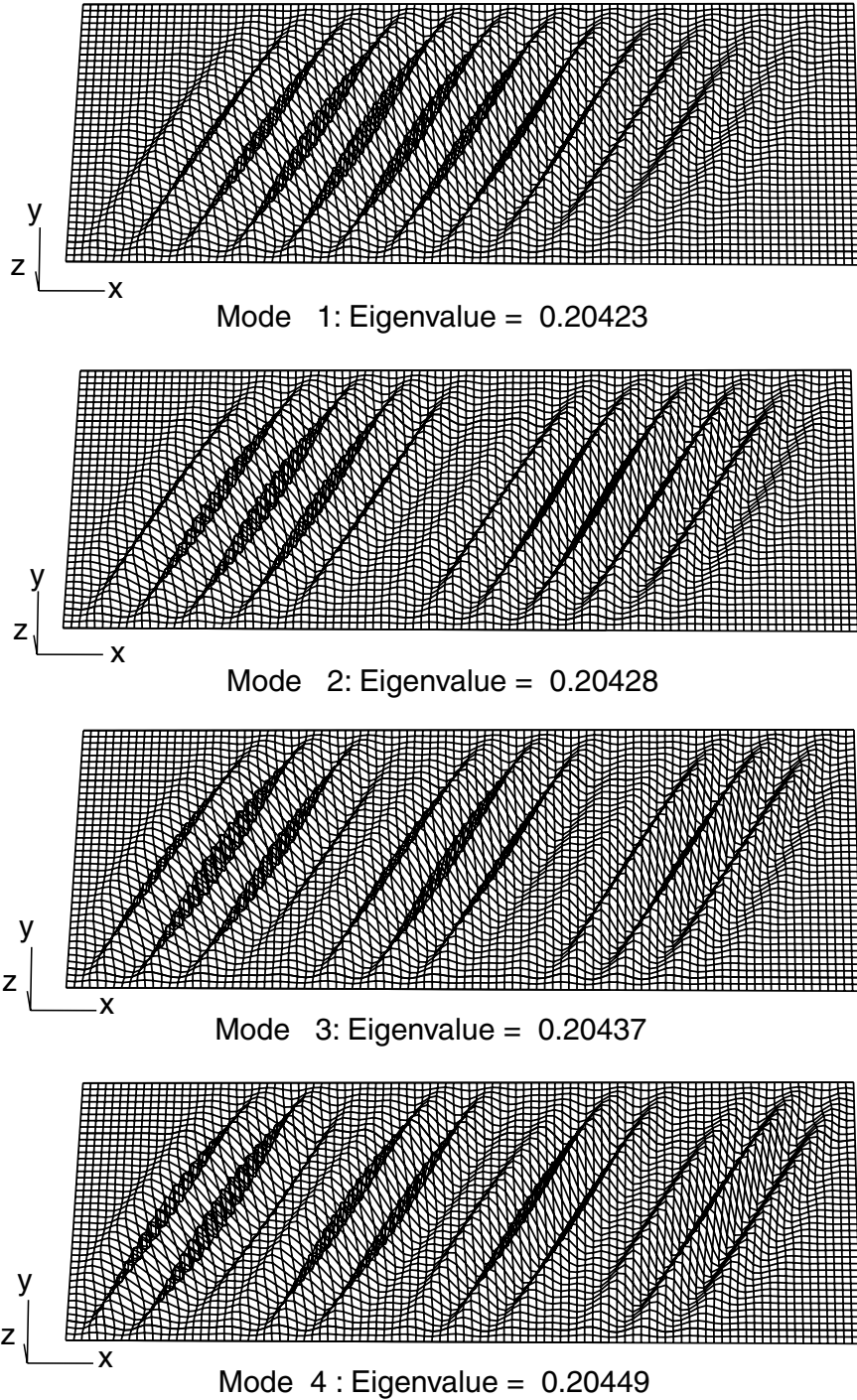
Figure 3. First four eigenmodes with eigenvalue > 0.2 , for membrane is shear.
