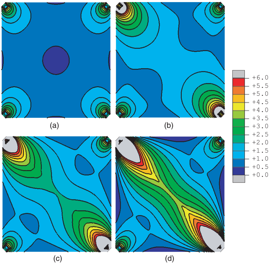
Figure 19. Contours of major midplane principal stress (in \text{N/mm}^2 ) obtained from thin-shell model for (a) T_1 = T_2 = 5 \text{ N} ; (b) T_1 = 10 \text{ N} , T_2 = 5 \text{ N} ; (c) T_1 = 15 \text{ N} , T_2 = 5 \text{ N} ; (d) T_1 = 20 \text{ N} , T_2 = 5 \text{ N} .
