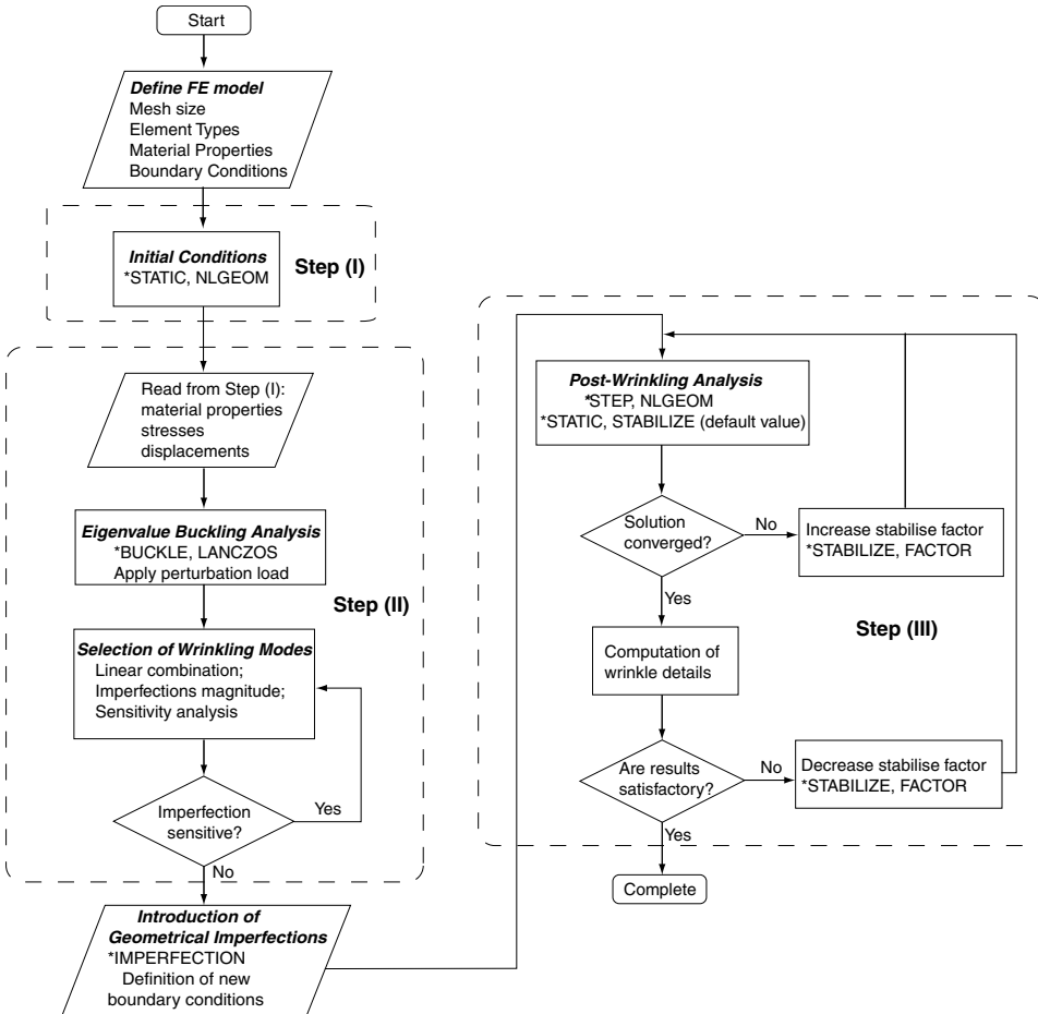
Figure 1. Flowchart for wrinkling analysis using thin shell model.
