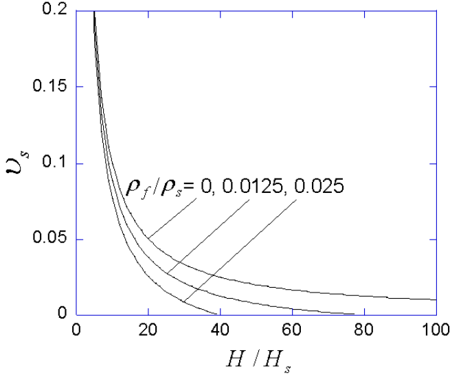
Figure 2: Volume fraction of steel versus normalized core thickness
