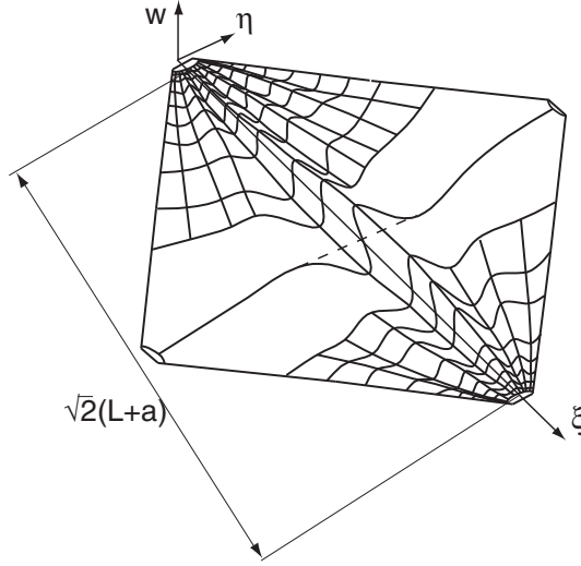
Figure 13. Wrinkle pattern for T_1/T_2 \geq 1/(\sqrt{2} - 1) .
