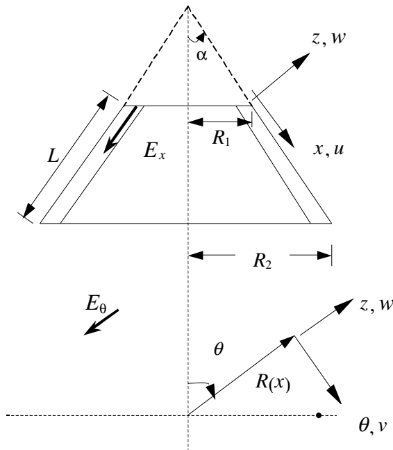
Figure 1. Geometry and notation of laminated conical shell.
