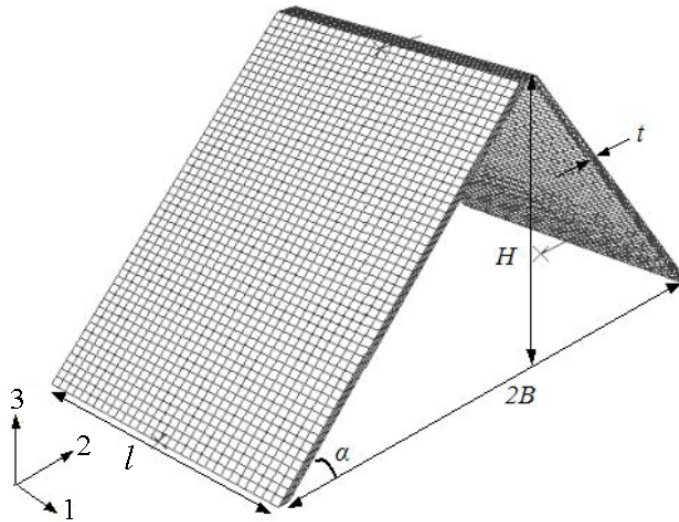
(b) Folded core geometry
