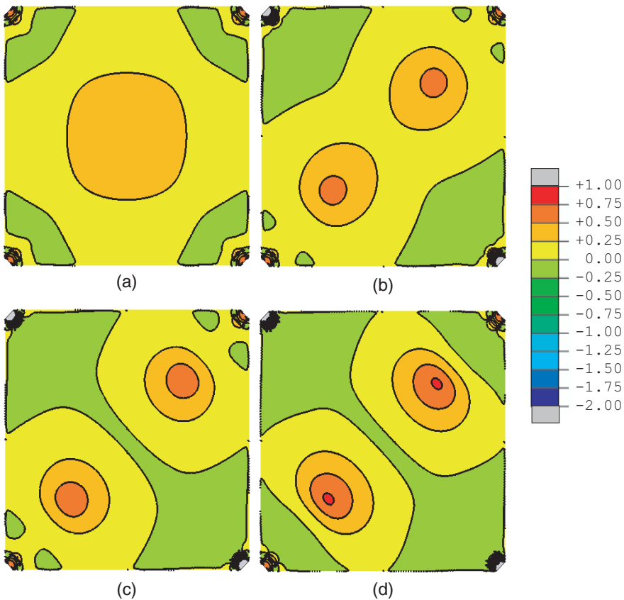
Figure 20. Contours of minor midplane principal stress (in \text{N/mm}^2 ) obtained from thin-shell model for (a) T_1 = T_2 = 5 \text{ N} ; (b) T_1 = 10 \text{ N} , T_2 = 5 \text{ N} ; (c) T_1 = 15 \text{ N} , T_2 = 5 \text{ N} ; (d) T_1 = 20 \text{ N} , T_2 = 5 \text{ N} .
