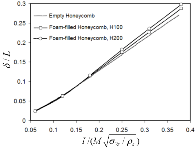
(a) The normalized maximum deflection of the top face sheet \delta/L
