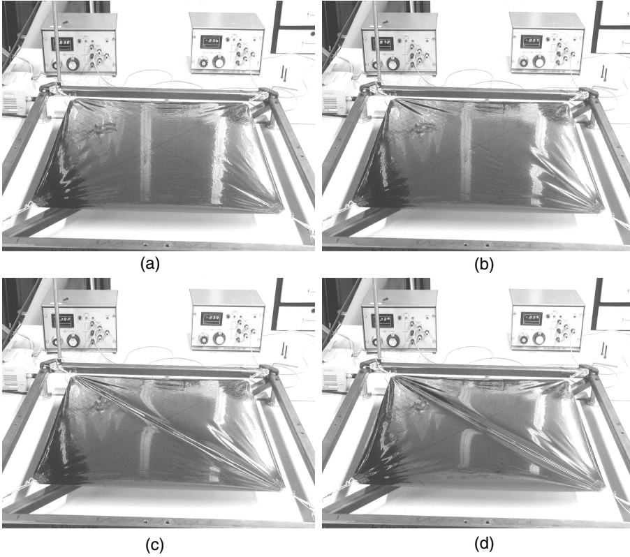
Figure 10. Wrinkle pattern in 0.025 mm thick square Kapton ® membrane for (a) T_1/T_2 = 1 , (b) T_1/T_2 = 2 , (c) T_1/T_2 = 3 and (d) T_1/T_2 = 4 .
