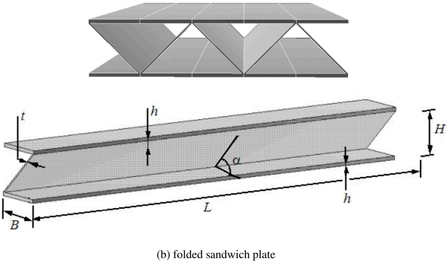
Figure 1: Schematic diagram of sandwich plate core configuration and corresponding computation model of sandwich panel (the polymeric foam components are not shown)
