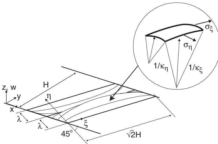
Figure 5. Perspective view of a single wrinkle.
