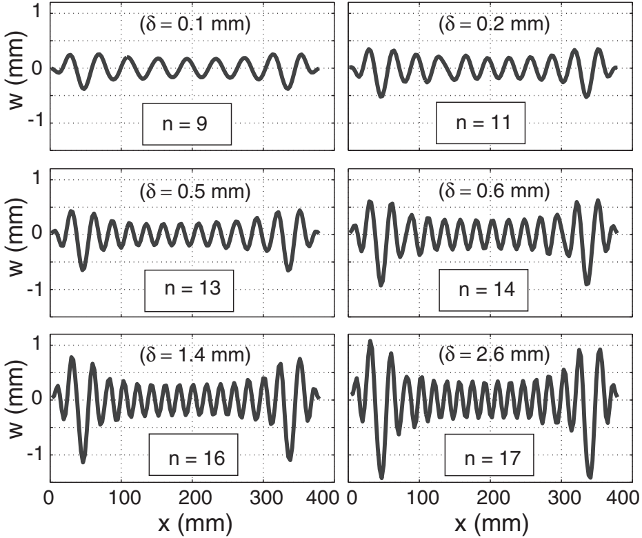
Figure 9. Mid-height cross-sections for different \delta 's.
