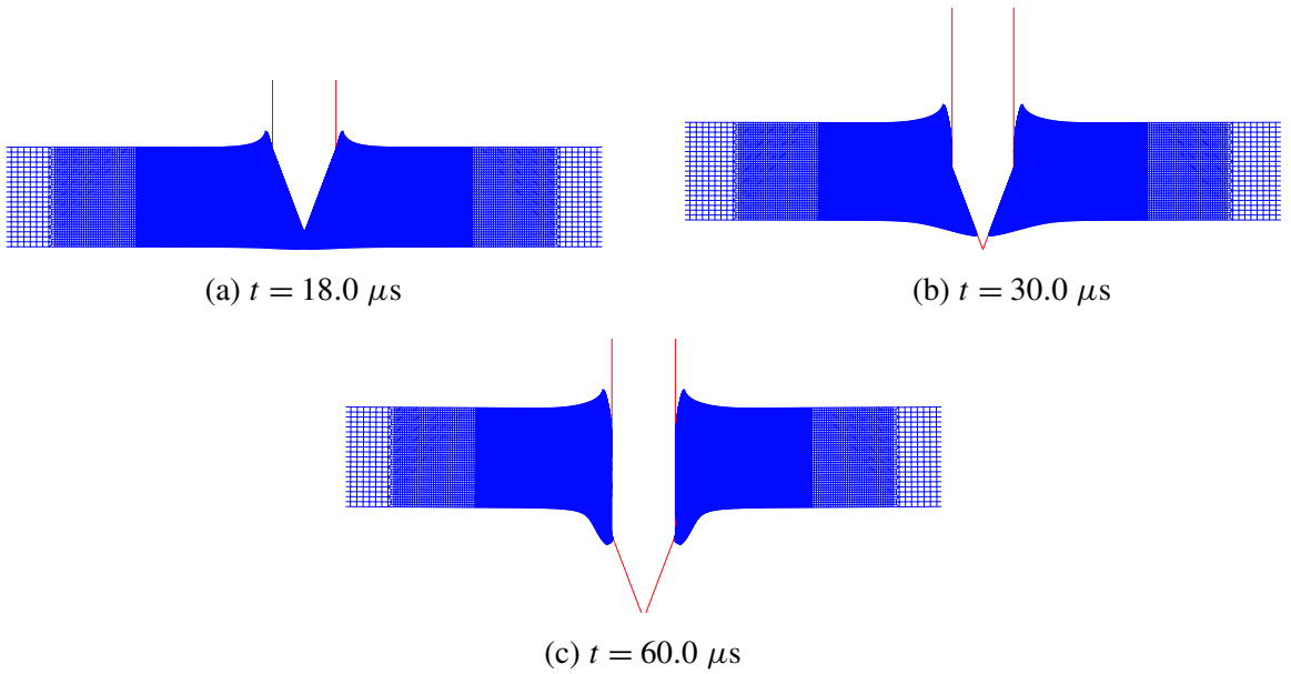
Figure 18. Perforation of monolithic shield impacted by a light, conical-nose projectile at V_0 = 600.0 \text{ m/s} .
