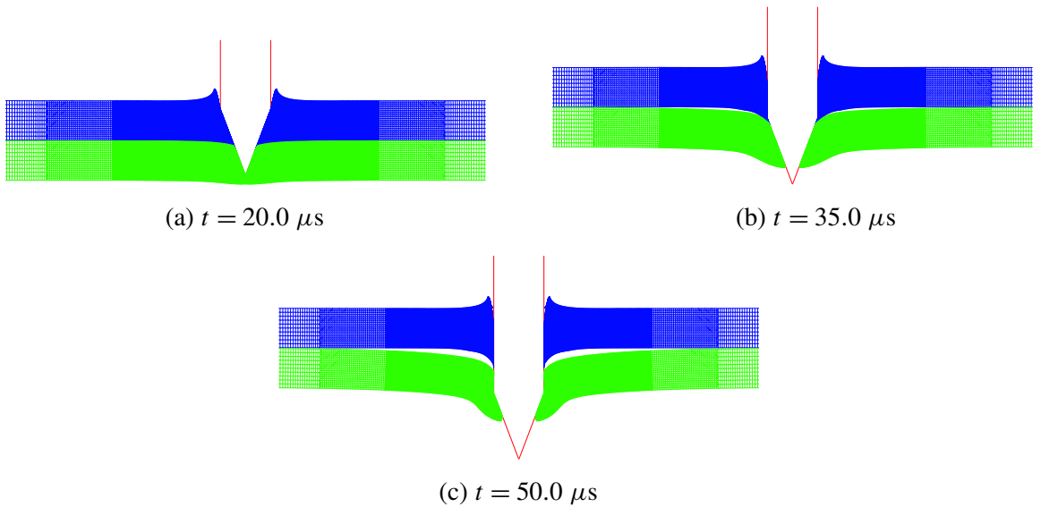
Figure 19. Perforation of double-layered shield with plates in contact impacted by a light, conical-nose projectile at V_0 = 600.0 \text{ m/s} .
