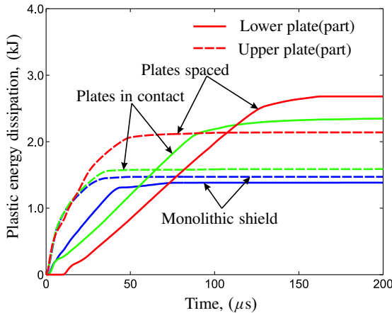
Figure 8. Time history of plastic energy dissipation of three shields at V_0 = 285.4 m/s.
