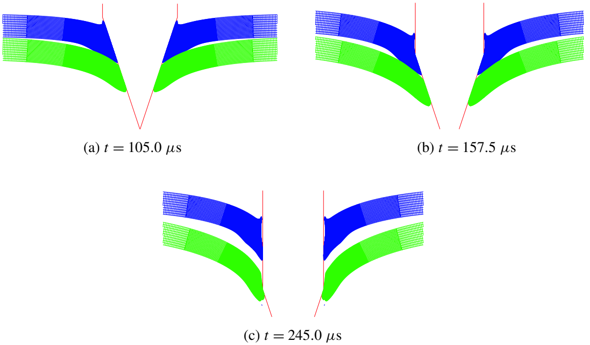
Figure 11. Perforation of double-layered shield with plates in contact impacted by a heavy, conical-nose projectile at V_0 = 317.9 m/s.
