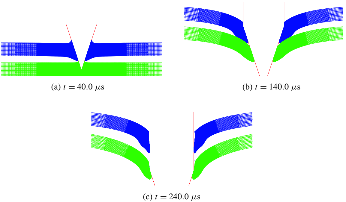
Figure 12. Perforation of double-layered shield with plates spaced impacted by a heavy, conical-nose projectile at V_0 = 317.9 m/s.
