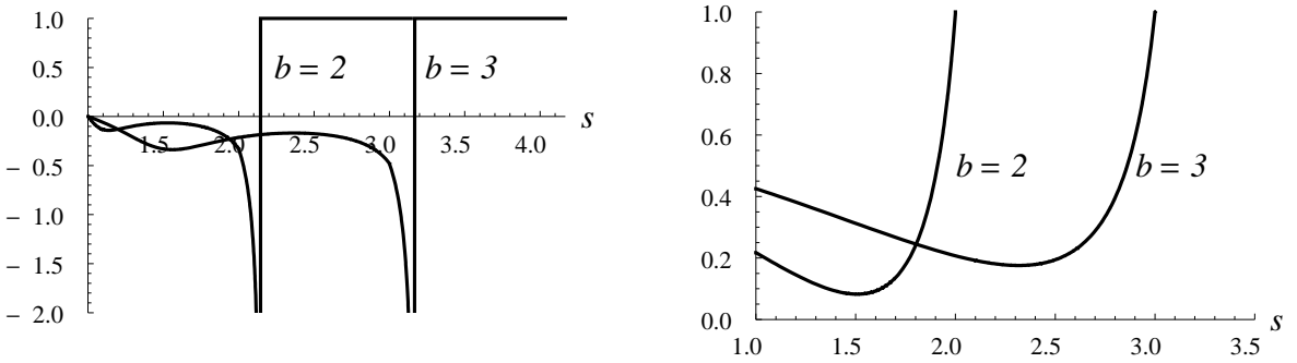
Figure 1. Graph of G_1(s) - H(c - s)B\sqrt{(c - a)/(c - s)} on the left and of G_2(s) on the right for a = 1, b = 2.0, 3.0, and c \approx 2.14, 3.17, respectively. The function G_1(s) - H(c - s)B\sqrt{(c - a)/(c - s)} involves a square root singularity and sign switch at s = c = 1/c_R, while G_2(s) is always positive.
