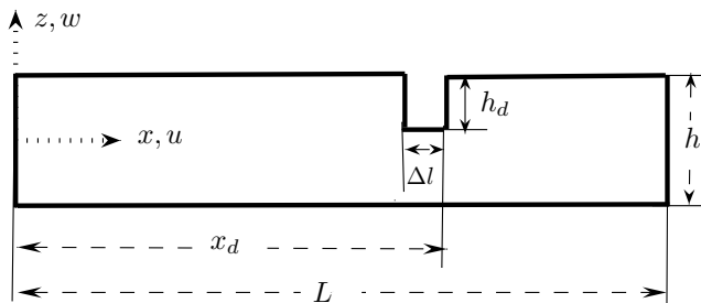
Figure 1. Beam geometry.
