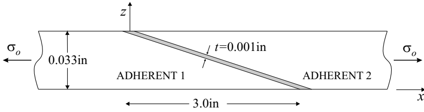
Figure 7. Schematics of the scarf joint.
