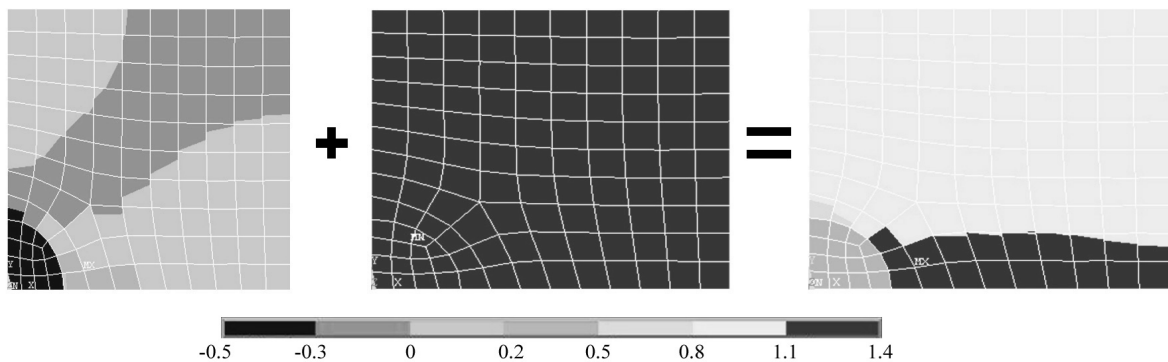
Figure 3. Fluctuation of strain, homogeneous strain, and total strain.
