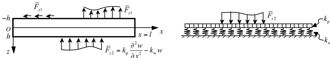
Figure 1. Left: geometry, coordinate system and loading condition of a beam resting on elastic foundations. Right: Pasternak foundation and beam foundation.
