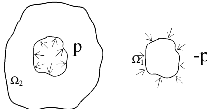
Figure 8. A region subjected to eigenstrain produces interfacial stress vector.
