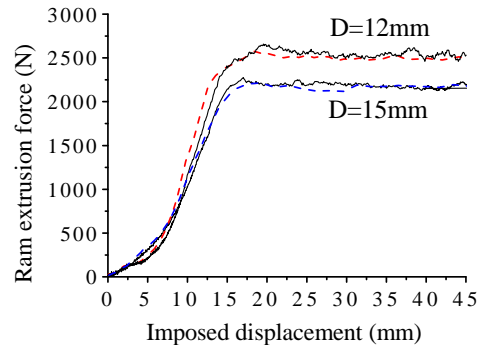
Figure 9. Curves of experimental (solid) and predicted (dashed) extrusion load versus imposed displacement ( L/D = 0.83 and V = 0.2 mm/s).
