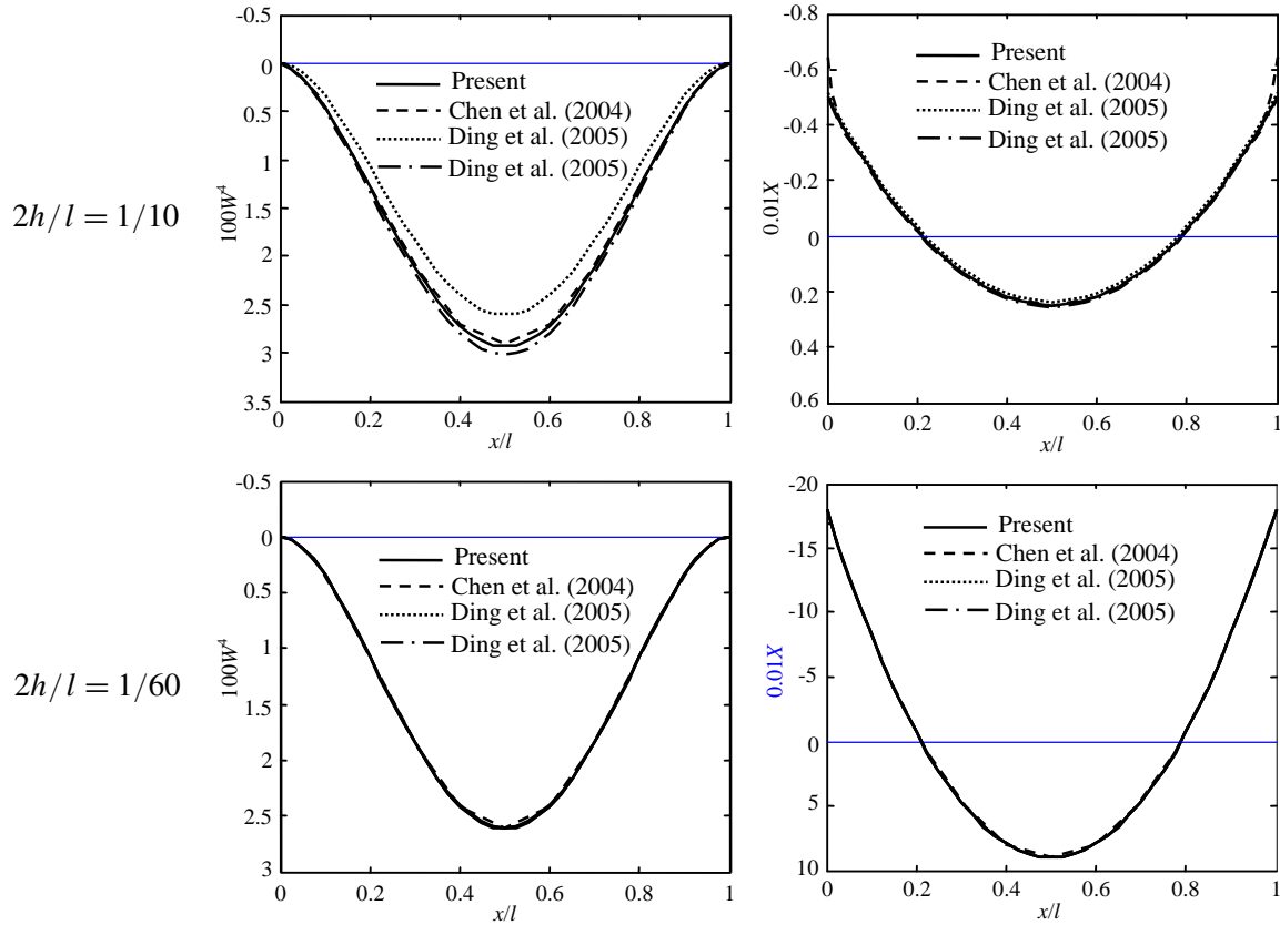
Figure 2. Deflection curves W(x, 0) and longitudinal axial normal stresses X(x, h) for CC beams without elastic foundations ( K_w = K_p = 0 ).
