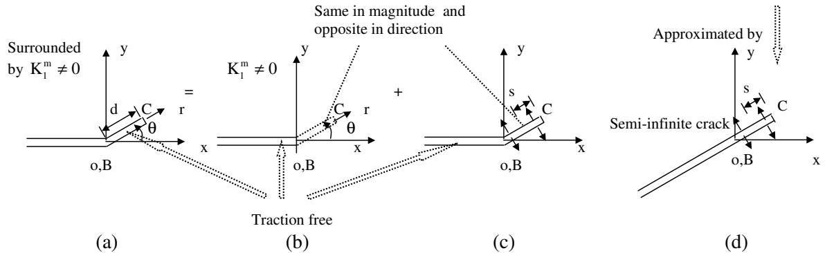
Figure 2. Superposition method in the kinked problem: (a) a kinked crack surrounded by the stress field defined by loading K_1^m , (b) a main crack with loading K_1^m , (c) a kinked main crack with loading on the kinked portion BC, and (d) a semiinfinite crack with loading on the interval BC.
