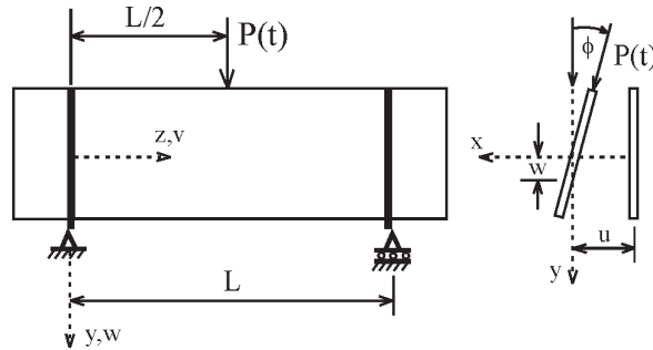
Figure 1. Thin rectangular beam subjected to stochastic excitation.
