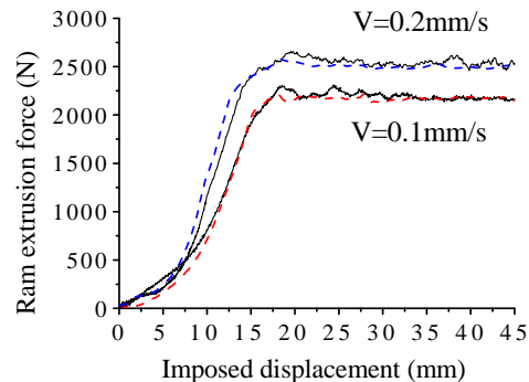
Figure 10. Curves of experimental (solid) and predicted (dashed) extrusion load versus imposed displacement ( L/D = 0.83 and L = 12 mm).
