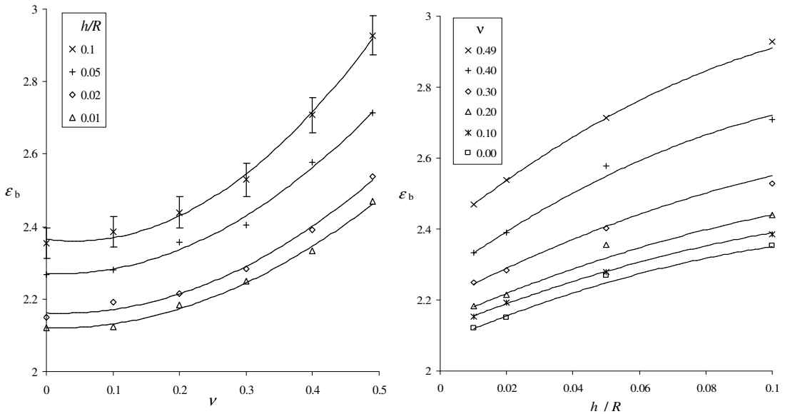
Figure 5. Left: Snap-through buckling point \epsilon_b versus Poisson's ratio \nu for a range of thickness-to-radius ratios ( h/R ) (left), and versus h/R for a range of values of \nu (right).
