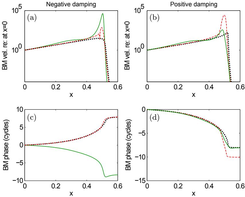
Figure 2. Steady state solutions of cochlea models for 1.6kHz harmonic stimulus: continuous green curves correspond to the time-delay model (2-5), dotted black lines correspond to the time-delay model with \tau(x) = 0 , and dashed red lines corresponds to the feed-forward model (2-10). The damping parameter is \zeta_0 = -0.06 for the left column and \zeta_0 = 0.01 for the right column.
