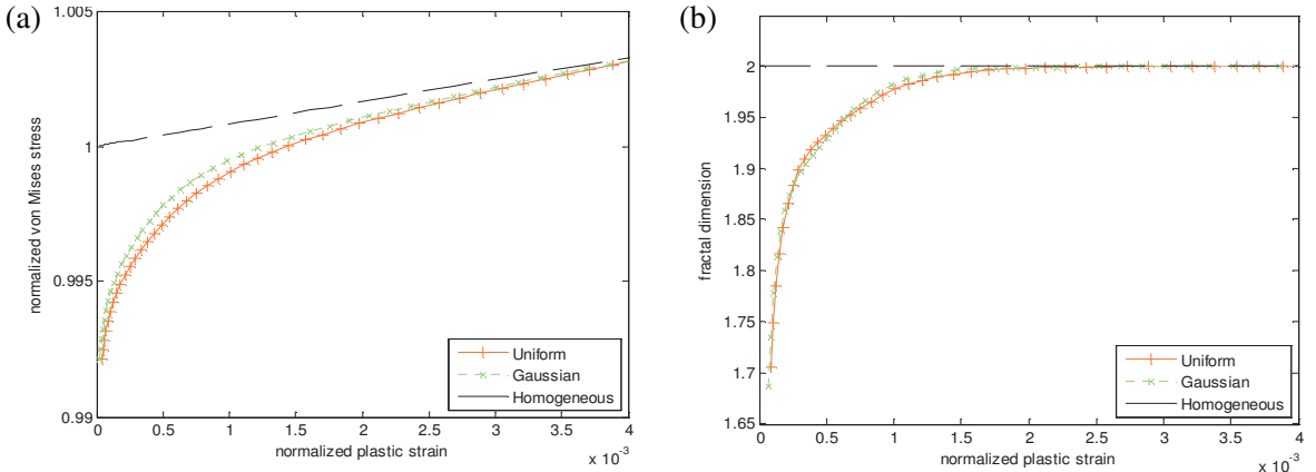
Figure 3. Comparison of elastic-plastic transitions for uniform and Gaussian random material distributions: (a) averaged stress~strain; (b) fractal dimension of the plastic set versus strain.
