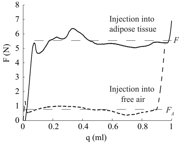
Figure 7. Force F versus the volume of saline injected q using a 0.4 mm diameter hypodermic syringe with a cross head displacement rate of 0.1 \text{ mm s}^{-1} .
