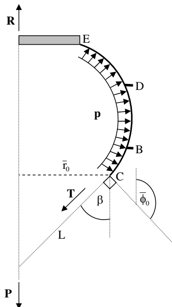
Figure 2. The basic parachute model.
