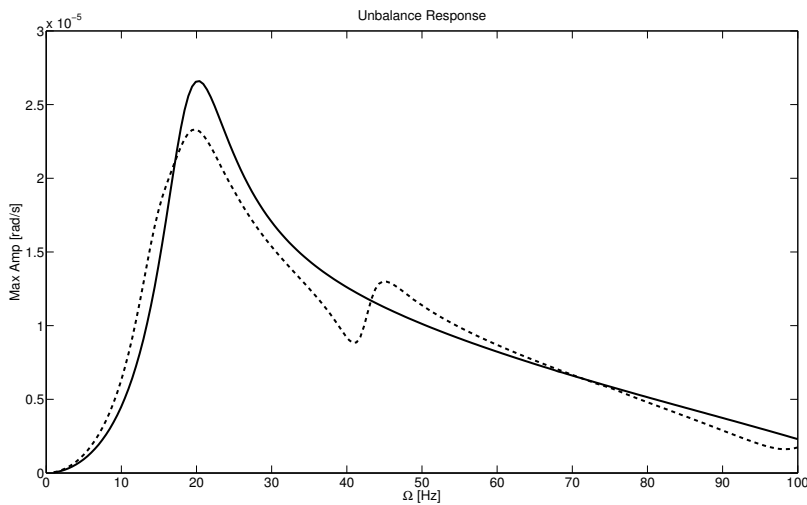
Figure 19. Unbalance response of linearized model (solid line) and nonlinear model (dashed line).
