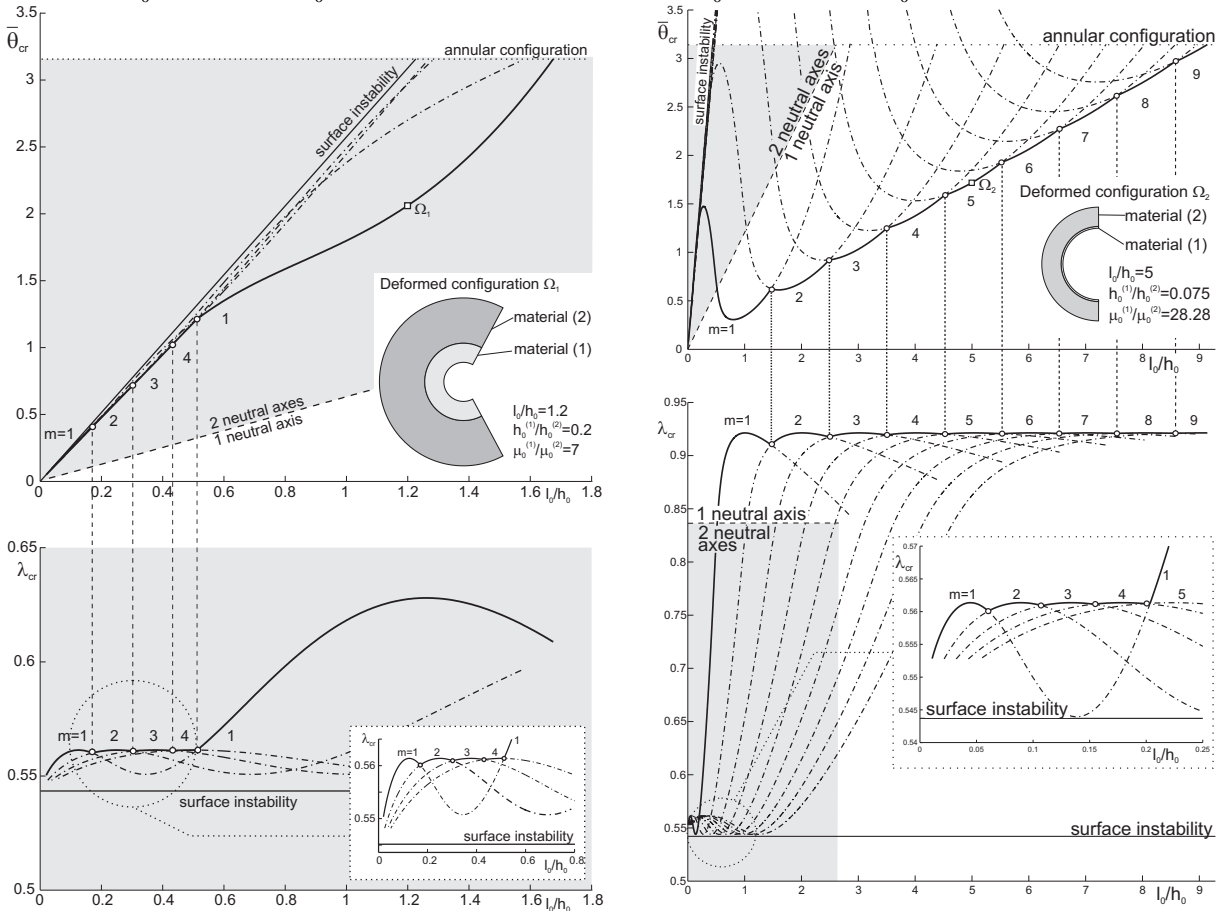
Figure 3. Critical angle \bar{\theta}_{cr} and critical stretch \lambda_{cr} (evaluated at the internal boundary, r = r_i^{(1)} ) versus aspect ratio l_0/h_0 for a Mooney–Rivlin bilayer coated with a stiff layer and subject to bending with h_0^{(1)}/h_0^{(2)} and \mu_0^{(1)}/\mu_0^{(2)} as indicated above the graphs. The stiff layer is located at the side in compression. In each plot, a small circle denotes a transition between two integer values of m (the parameter which sets the circumferential wavenumber). In the lower plots, the insert contains a magnification of the region where bifurcations occur at low l_0/h_0 . Two neutral axes occur in the region marked gray.
