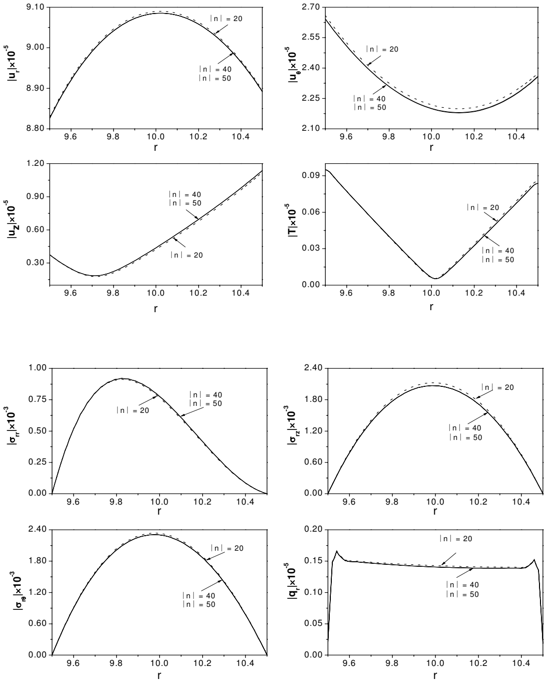
Figure 9. Through-the-thickness dependence of numerically calculated quantities for a silicon nitride cylinder at \omega^* = 5.0 with |n| = 20, 40, 50 . The top two rows show the displacement components and the temperature distribution; the bottom two rows, the stress components and the heat flux.
