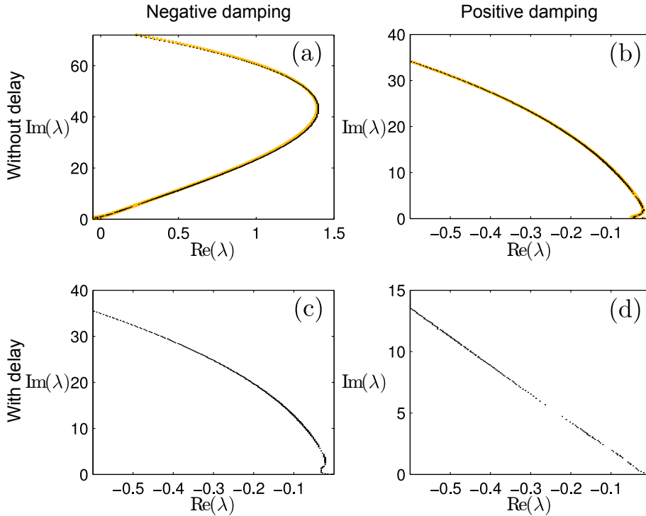
Figure 4. Stability of the time-delay model. Black points show the characteristic roots of (2-5), computed from the characteristic function \det M = 0 , without delay (top) and with delay (bottom). In the nondelay case, the roots are also computed with a direct method using Chebyshev collocation, as a check; these values are indicated with color dots. The damping parameter is \zeta_0 = -0.06 for the left column and \zeta_0 = 0.01 for the right column.
