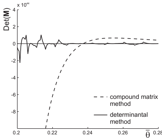
Figure 2. The compound matrix method (dashed line) against the determinantal method (solid line): \det(\mathbf{M}) is evaluated at different angles \bar{\theta} , for l_0/h_0 = 0.1 , h_0^{(1)}/h_0^{(2)} = (1 \text{ mm})/(5 \text{ mm}) and \mu_0^{(1)}/\mu_0^{(2)} = (7 \text{ N/mm}^2)/(1 \text{ N/mm}^2) . Bifurcation corresponds to the vanishing of \det(\mathbf{M}) ; note the spurious oscillations of the latter method.
