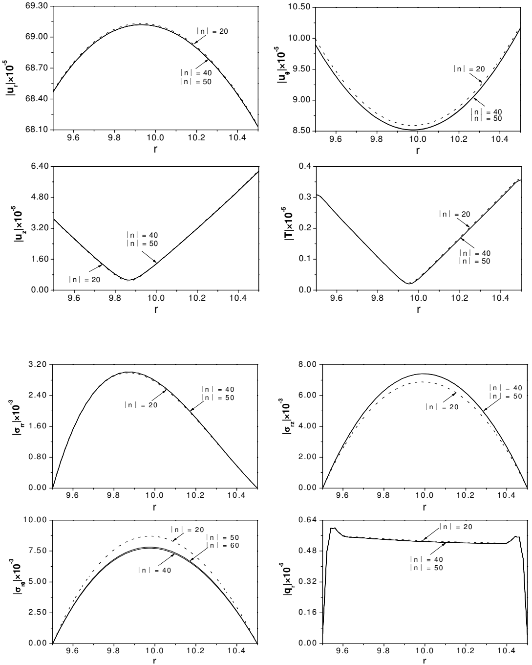
Figure 8. Through-the-thickness dependence of numerically calculated quantities for a silicon nitride cylinder at \omega^* = 3.0 with |n| = 20, 40, 50 . The top two rows show the displacement components and the temperature distribution; the bottom two rows, the stress components and the heat flux.
