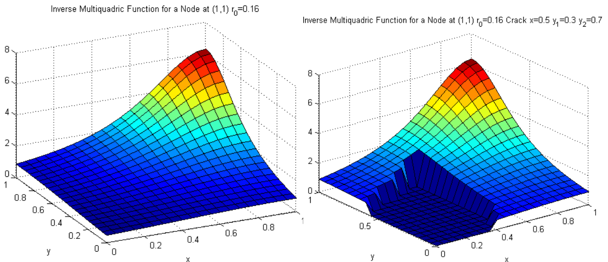
Figure B.2. IMQ basis function of the corresponding node on a four-node element, with and without a crack inside the horizon.
