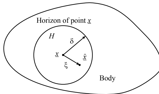
Figure 1. Each point \underline{x} in the body \Omega interacts directly with the points \underline{\hat{x}} in the circular disc H(\underline{x}) through bonds.
