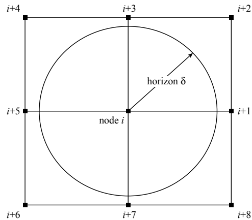
Figure B.1. The horizon of one node over four elements, the stiffness density of the node i is calculated through (33) and (34).
