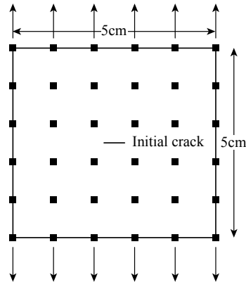
Figure 9. A 5 cm \times 5 cm plate under tension, including an initial crack in the center.
