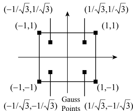
Figure A.1. Gaussian quadrature of 2 \times 2 points of weight 1.
