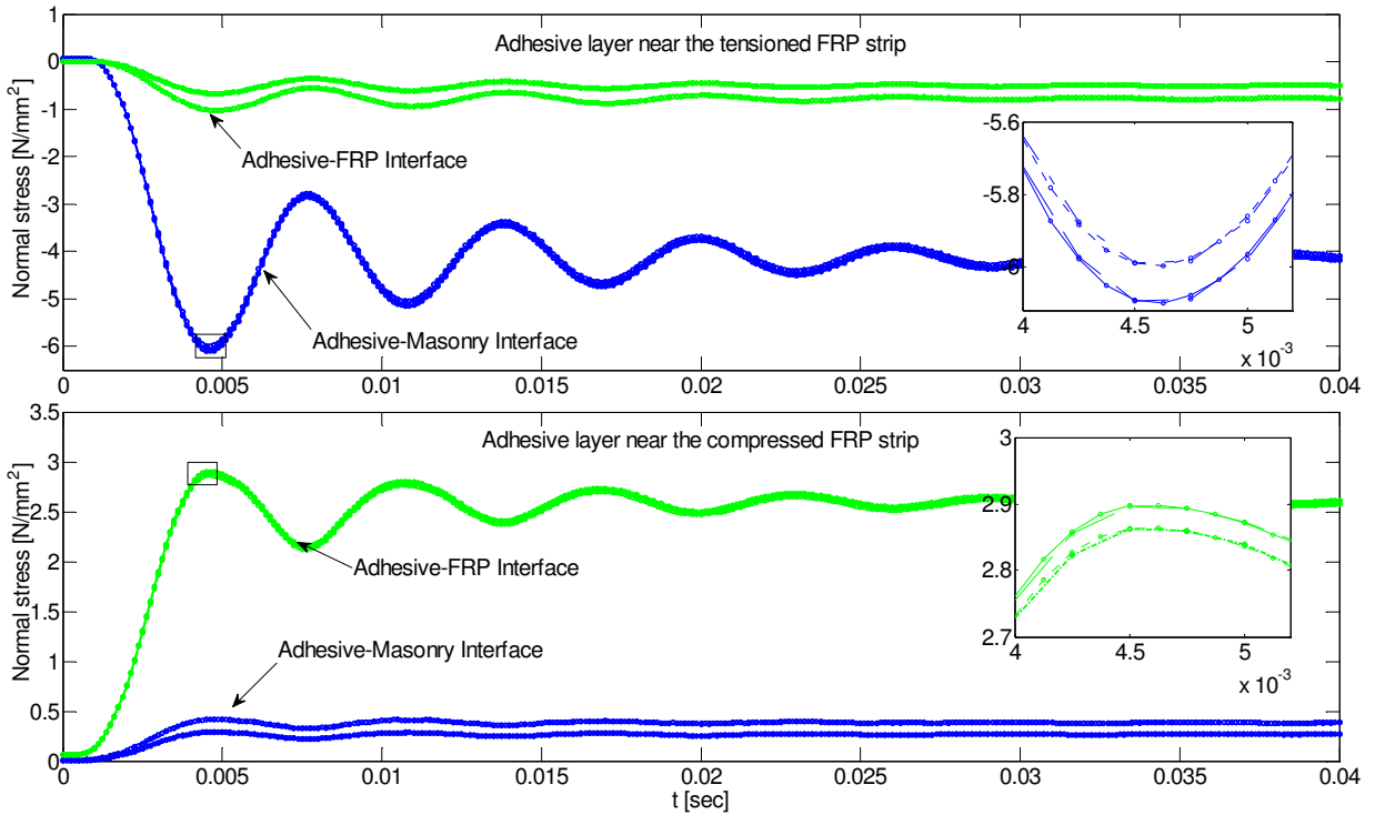
Figure 11. Out-of-plane normal stresses at x = 415 mm versus time. Legend: - · - · - Mesh M2T1; - - - Mesh M3T1; · · · · · Mesh M2T2; — Mesh M3T2, o time steps.
