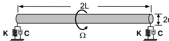
Figure 5. A bearing-supported uniform shaft, where \Omega is the spinning speed.
