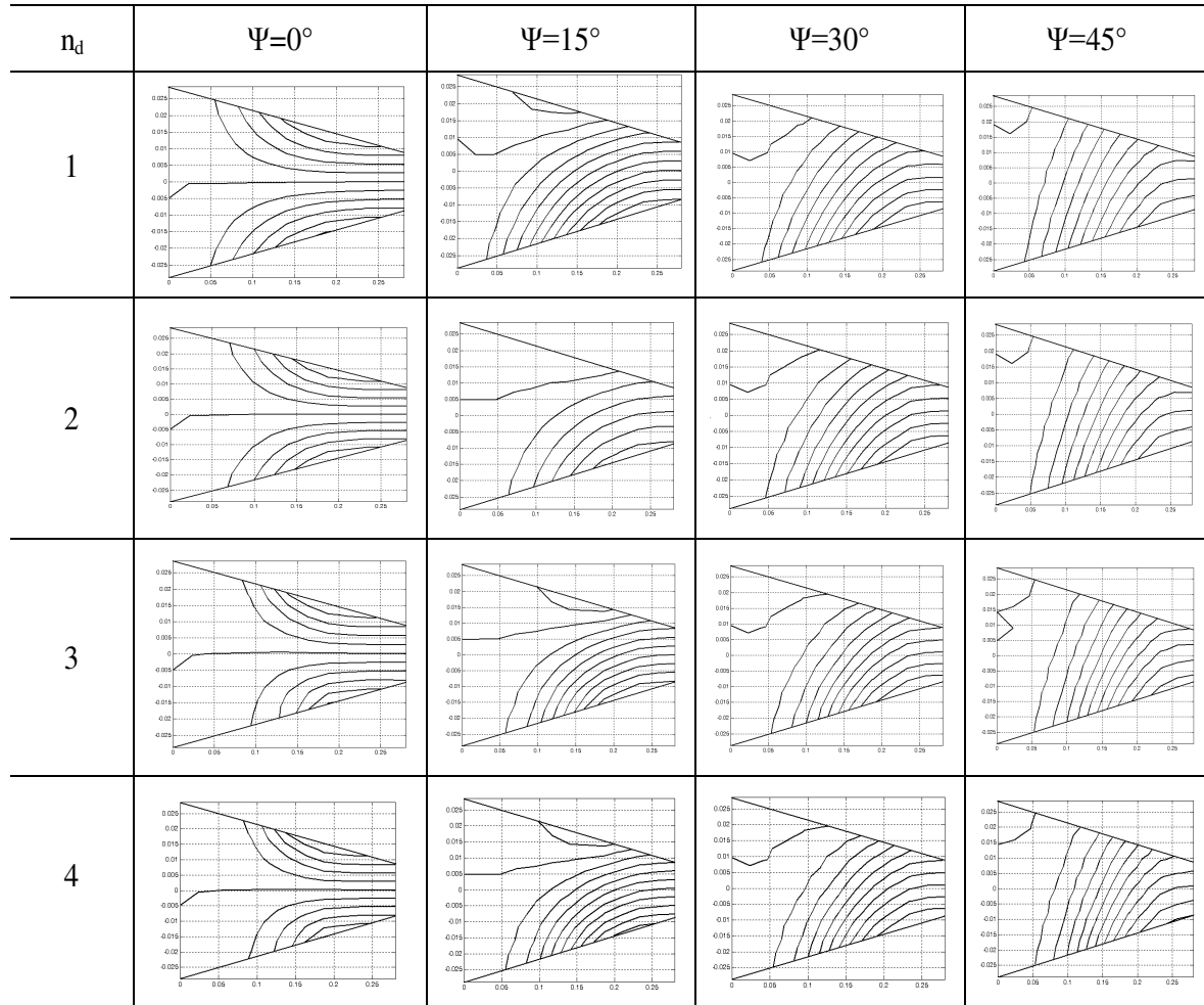
Figure 6. Effect of twist and number of delaminations on mode shapes for NDFP of graphite-epoxy bending-stiff delaminated composite conical shells, considering n = 8 , h = 0.0004 , s/h = 1000 , a/L = 0.33 , d/L = 0.5 , L/s = 0.7 , \theta_0 = 45^\circ , and \theta_v = 20^\circ .
