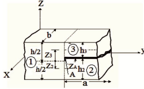
Figure 2. Plate elements at a delamination crack tip.
