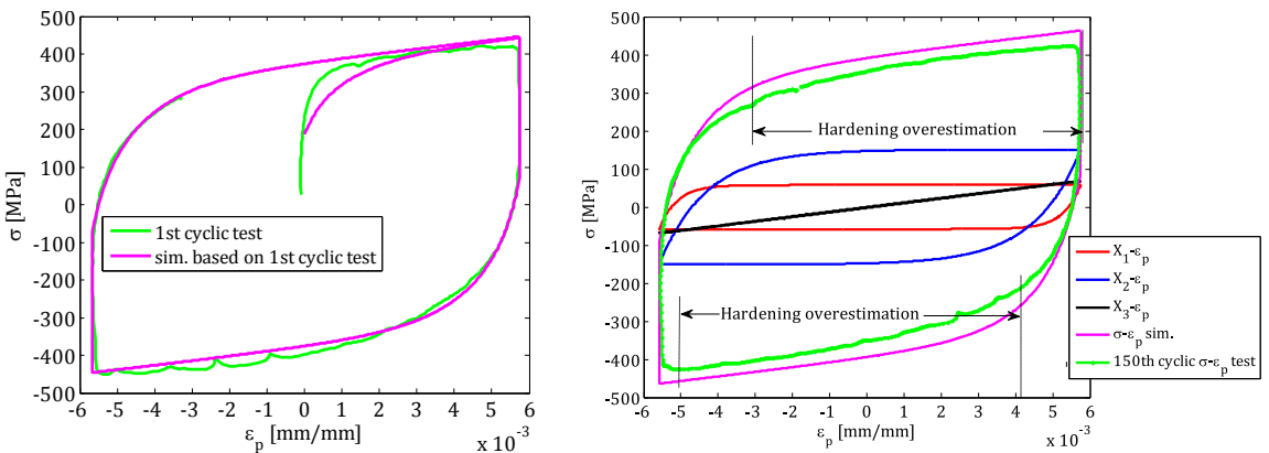
Figure 8. Left: comparison between the simulated \sigma - \epsilon_p response and the first cyclic test. Right: comparison between the 150th cyclic test and \sigma - \epsilon_p response simulated based on the parameters from Table 4.
