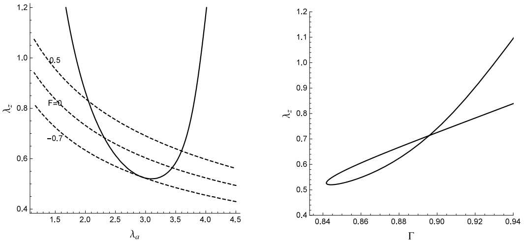
Figure 3. Solution of the bifurcation condition \Omega_u(\lambda_a, \lambda_z) = 0 , when the Ogden material is used, for a rotating tube with A = 0.8 and P = 0 in terms of (\lambda_a, \lambda_z) (left) and (\Gamma, \lambda_z) (right). The dashed lines represent the loading paths with F = 0, 0.5, -0.7 .
