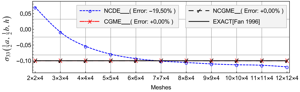
Figure 7. Comparison of stress \sigma_{33}(\frac{1}{2}a, \frac{1}{2}b, h) .
