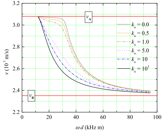
Figure 7. Dispersion curve for the antisymmetric part for k_\varphi = 10^7 F/m 2 and different values of k_u .
