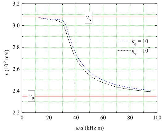
Figure 8. Dispersion curve for the antisymmetric part for k_u = 0.5 GPa/m and different values of k_\varphi .
