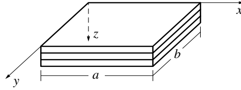
Figure 1. The geometry and coordinate system of the laminated plate.
