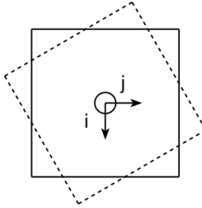
Figure 1. Composite figure associated with D_4 \cap \mathbf{r}D_4\mathbf{r}^t , where \mathbf{r} = \mathbf{Q}(\mathbf{k}; \pi/3) .
