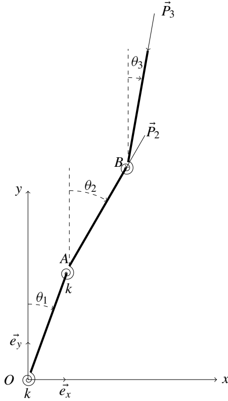
Figure 3. Three degree of freedom discrete Leibholz system.
