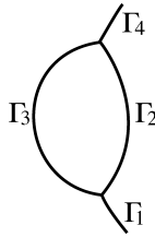
Figure 16. Case (2, 1) models cases (-2, -1) , (-1, -2) and (1, 2) .
