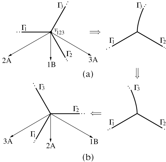
Figure 8. A close-up of v_{123} as it turns one notch counterclockwise. In (a), m = 0 and 2A < 1B < 3A ; on the right, 3A = +\infty . In (b), m = 1 and 3A < 2A < 1B ; 3A = -\infty on the right.
