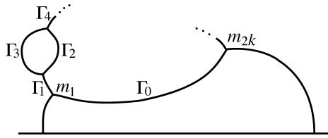
Figure 21. If the (2, 1) leaf is the leftmost leaf, then all other leaves are near graph.
