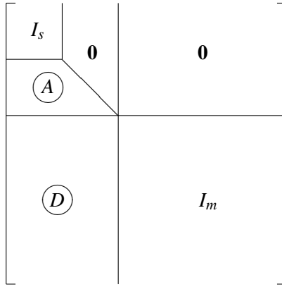
Figure 1. Shape of O_{GL_n/\tilde{P}_s}^- .
