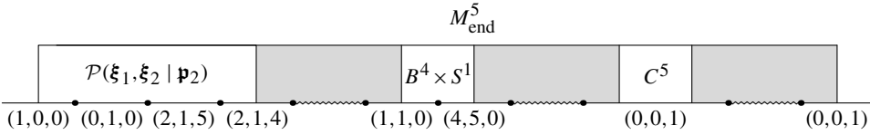
Figure 5. An example of the decomposition of the domain of outer communication described in Theorem B. The black hole horizons, represented by jagged intervals, are deformation retracts of the gray areas. In the leftmost piece of the decomposition, \xi_1 is formed by a disk bundle over L(5, 2) with Euler class determined by 1, while \xi_2 is formed by a disk bundle over L(2, 1) with Euler class 0; the plumbing vector is \mathbf{p}_2 = (1, 0, 2) . The remaining pieces include a neighborhood of a corner B^4 \times S^1 , a region centered on the interior of an axis rod C^5 = [0, 1] \times D^2 \times T^2 , and the asymptotic end M_{\text{end}}^5 which is homeomorphic to \mathbb{R}_+ \times S^3 \times S^1 .
