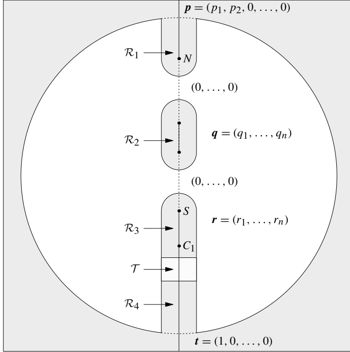
Figure 2. The various regions used in the construction of the model map. Axis rod structures are represented by p , q , r , and t , while horizon rods are indicated by dashed lines.
