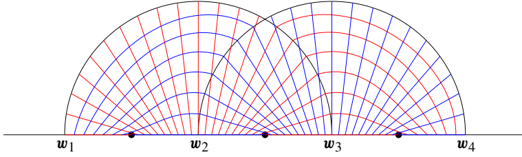
Figure 4. We have \mathbf{w}_1 = \mathbf{e}_1 , \mathbf{w}_2 = \mathbf{e}_2 , \mathbf{w}_3 = (q_1, r_1, p_1) , and \mathbf{w}_4 = q_2\mathbf{w}_2 + r_2\mathbf{w}_3 + p_2\mathbf{p}_2 in accordance with (6-5a). The diagram shows a toric plumbing of two disk bundle-torus products \xi_1 and \xi_2 over lens spaces L(p_1, q_1) and L(p_2, q_2) , along plumbing vector \mathbf{p}_2 . The fibers of \xi_1 are given by rays emanating from \mathbf{w}_2 , while the fibers of \xi_2 are given by rays emanating from \mathbf{w}_3 . Note that in the overlap, the fibers and sections switch roles between \xi_1 and \xi_2 .
