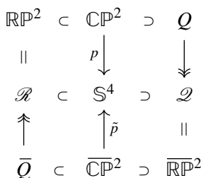
Figure 1. The two branched coverings of interest and their associated branch loci. The arrows marked \longrightarrow denote an unbranched 2-fold cover from a 2-sphere to a real projective plane.
