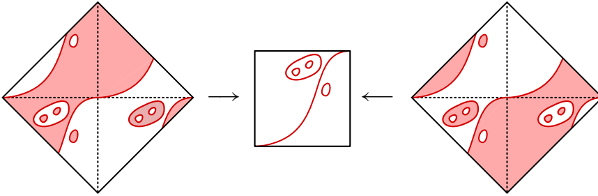
Figure 11. In the middle, a curve with real scheme \langle(1, 1), 1 \sqcup 1(2)\rangle . On the left and on the right, the two possible choices \bar{\Omega}_{\pm} .
