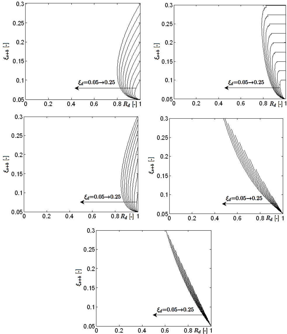
Figure 12. Design charts for different types of dampers: variation of \zeta_{s+b} with R_d ( \zeta_d = 0.05-0.25 ). Clockwise from top left: VL, VN, EP, FR, VE.
